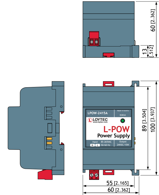
DIM025 LPOW-2415A
