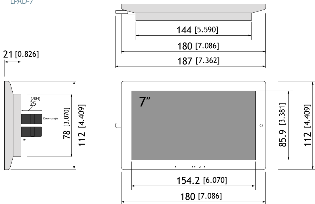
DIM068 LPAD-7
