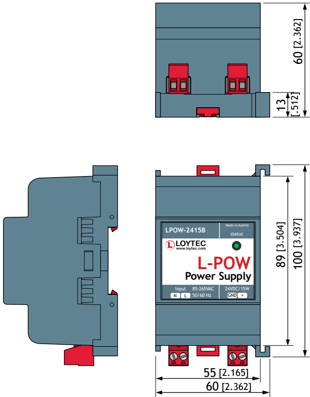
DIM026 LPOW-2415B
