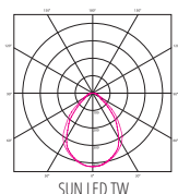
SUN LED TW
