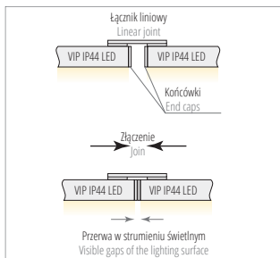
VIP IP44 LED - linia świetlna VIP IP44 LED - light line
