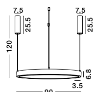
SONIK - 9010180 Sandy Black Aluminium LED Upside Light 40W CRI>90 Down Side Capability 30W Driver 100W 220-240V 3080Lm 3000K IP20 Beam Angle: 120° D: 90 W: 3.5 H: 120 cm
