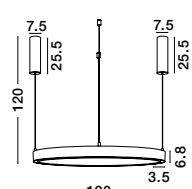
SONIK - 9010181 Sandy Black Aluminium LED Upside Light 55W CRI>90 Down Side Capability 40W Driver 100W 220-240V 3277Lm 3000K IP20 Beam Angle: 120° D: 120 W: 3.5 H: 120 cm
