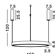
SONIK - 9010182 Sandy Black Aluminium LED Upside Light 65W CRI>90 Down Size Capability 50W Driver 100W 220-240V 4042Lm 3000K IP20 Beam Angle: 120° D: 150 W: 3.5 H: 120 cm
