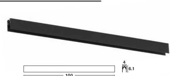
SURFACE - PENDANT APPLICATION
