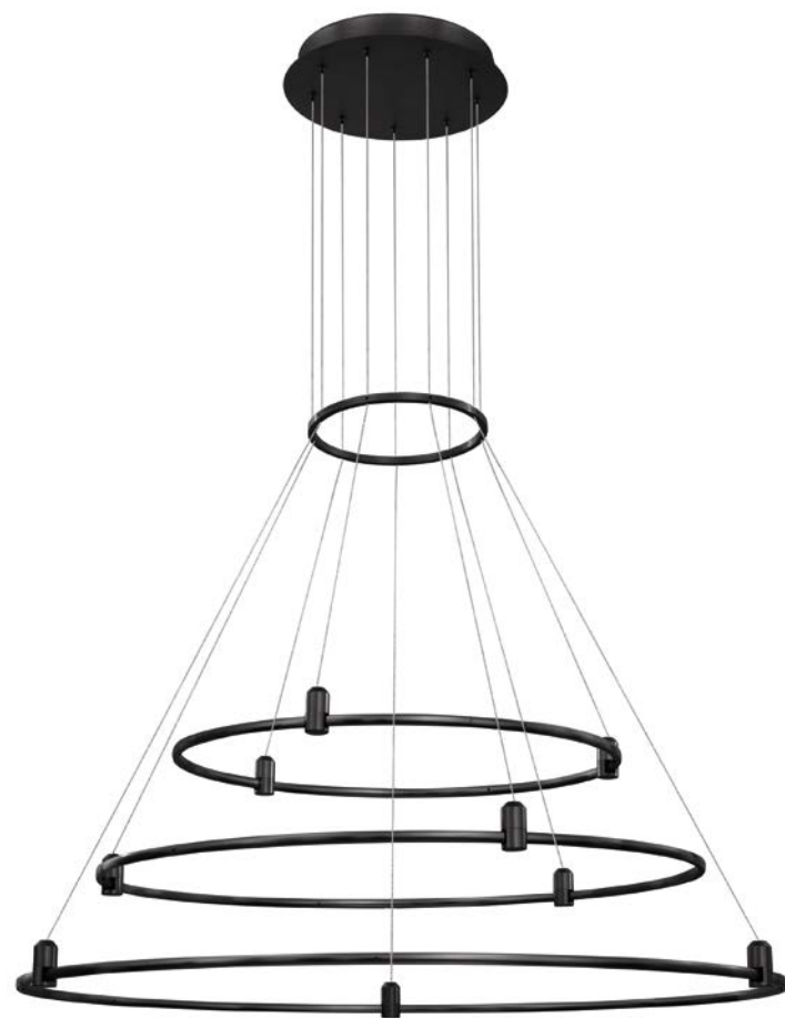
DION . 9028923 Magnetic Circular Structure Sandy Black Aluminium IP20 Included Driver 350 Watt AC220-240V Output 24V DC D1: 100 D2: 80 D3: 60 H: 200 cm
