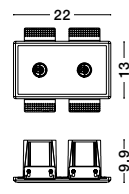
IMAGINE - 9492801 White Plaster, Aluminium & Acrylic Cut Out: 22.1 x 13.1 cm L: 22 W: 13 H: 9.9 cm
