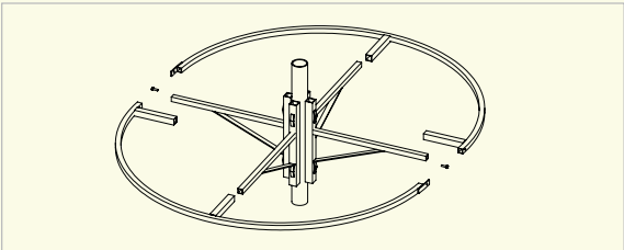
PIX02 / PIX03 Circular bracket for assembling your 3D decorations Inner diameter adjustable
