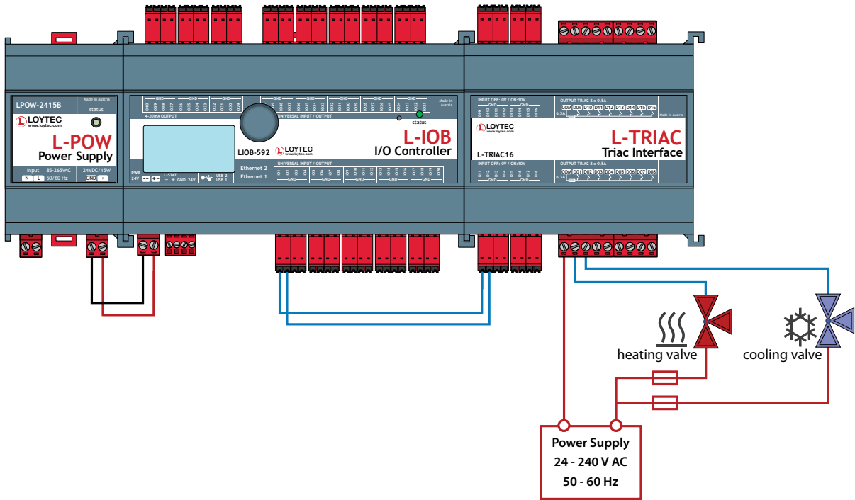
Wiring example:
