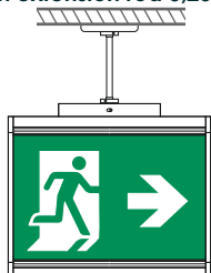
Ceiling mounting with extension rod 0,25-1m
