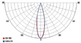
24° narrow beam angle with optional 24° lens
