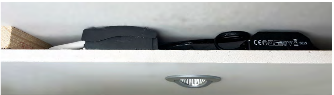
6 - The result: a compact installation with a swivelling spot, a dimmable power supply unit and the option of through-wiring in the ceiling cavity - ideal in refurbishment areas.
